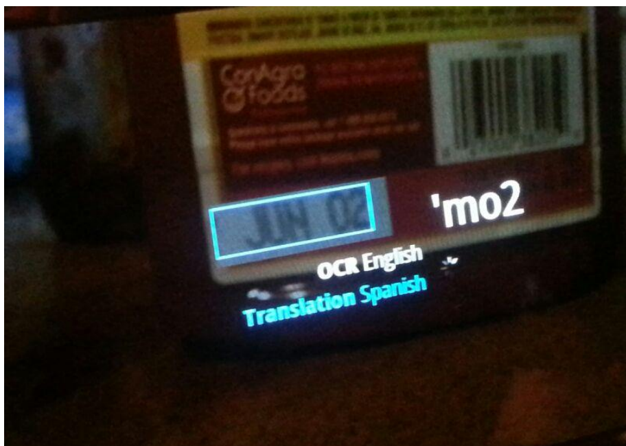
Figure 6.10 Performing OCR
