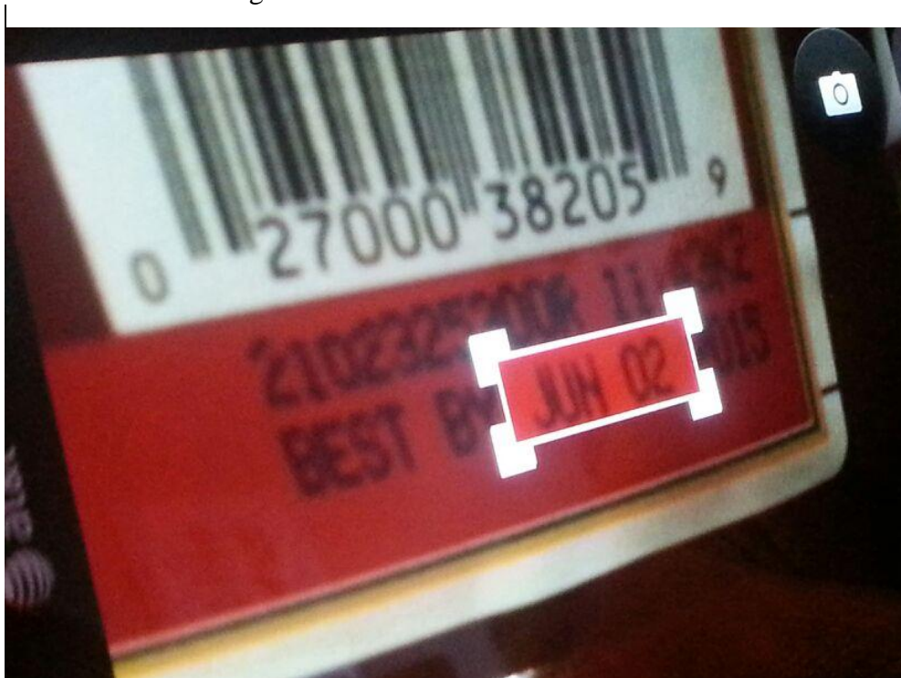
Figure 6.9 OCR Scanning
