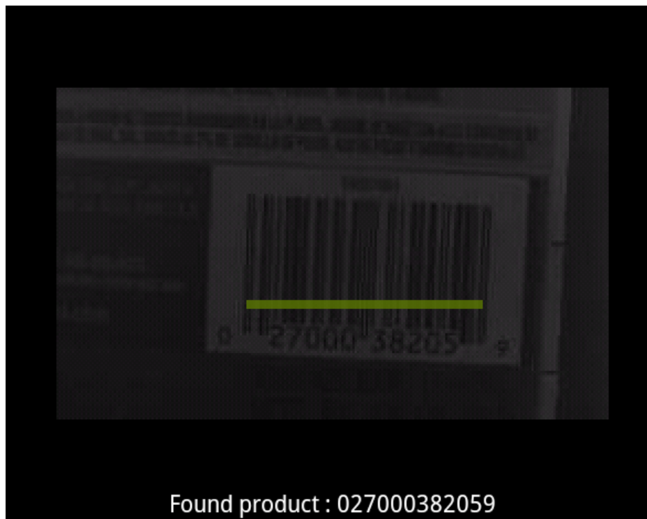
Figure 6.7 Barcode Found
